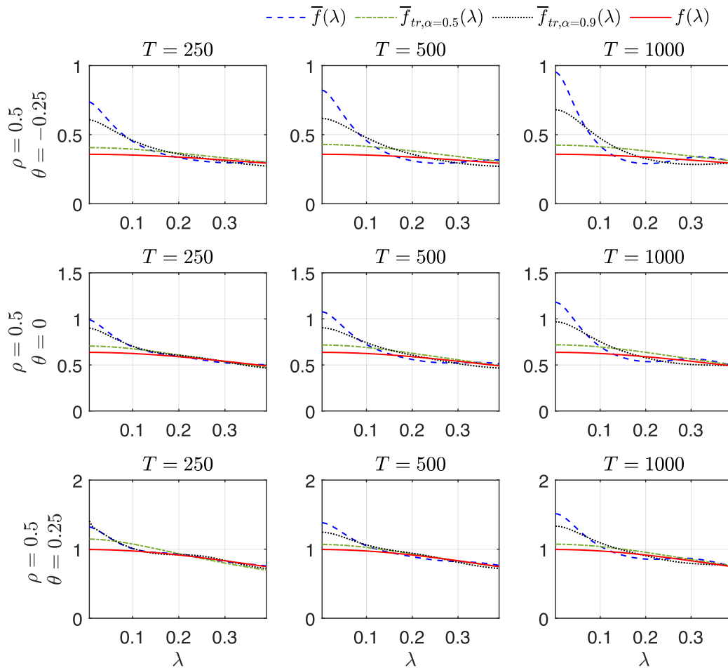
Figure 2. Average behavior of the autoregressive spectral density estimator over 10^4 Monte Carlo replications. The data are generated using y_t = m_t + x_t , t = 1, 2, \dots, T where m_t = 1.5 + 0.5\mathbf{I}_{\{t > T/2\}} , x_t = \rho x_{t-1} + \varepsilon_t + \theta \varepsilon_{t-1} where \rho = 0.5 , \theta \in \{-0.25, 0, 0.25\} and \varepsilon_t \sim \text{i.i.d. } \mathcal{N}(0, 1) . See Figure 1 for further details
